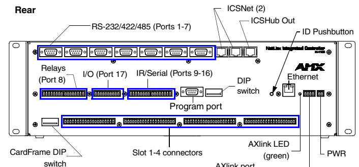
FIG. 2 NI-4100 rear connectors and components
